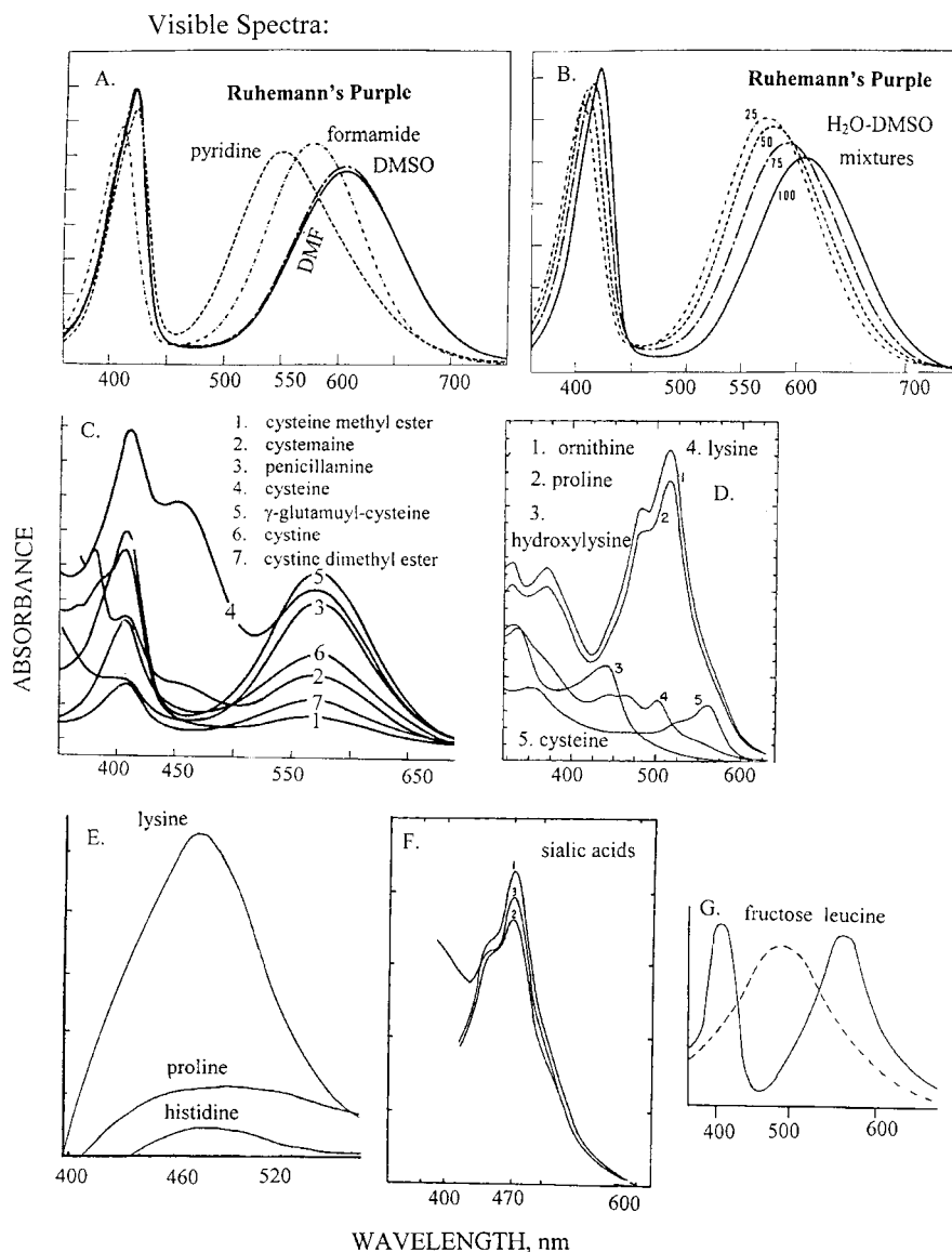
Figure 3. Absorption spectra: (A) Ruhemann's purple in different solvents, (B) Ruhemann's purple in DMSO–H 2 O solutions (4), (C) Ruhemann's purple derived from sulfur amino acids (37), (D) ninhydrin-ferric chromophores (124), (E) acid-ninhydrin chromophores (143), (F) sialic ( N -acetylneuraminic) acid–ninhydrin chromophores (163), (G) fructose-ninhydrin chromophore (142).
