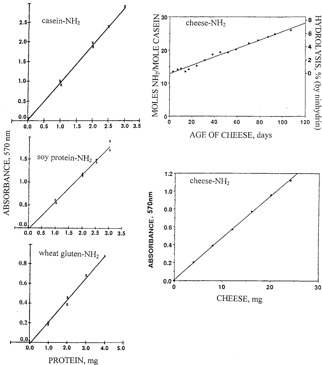
Figure 9. Linear relationships between ninhydrin color yields and concentrations of food proteins (7, 8).
